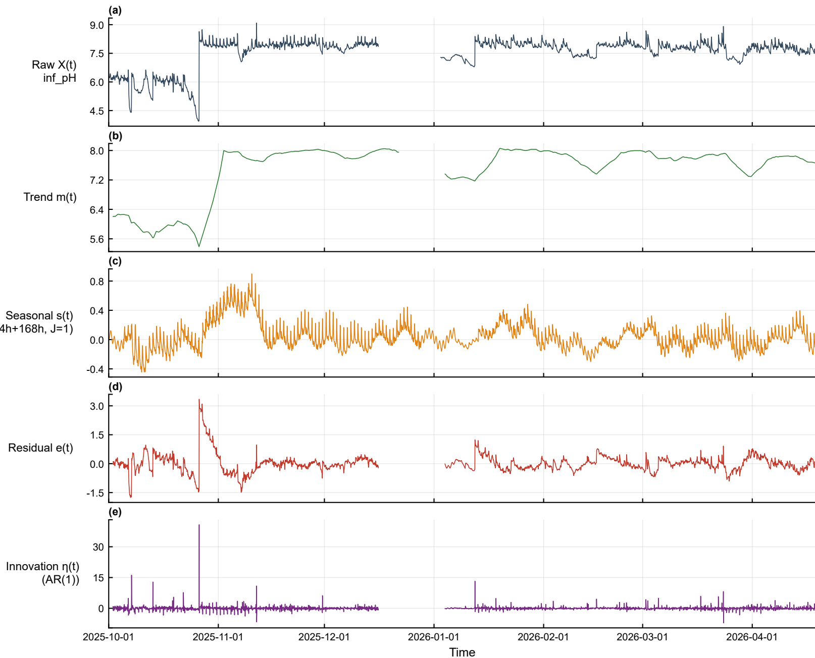
Multi-scale decomposition — inf_pH (influent, hour) [2025-10-01~2026-04-19]
